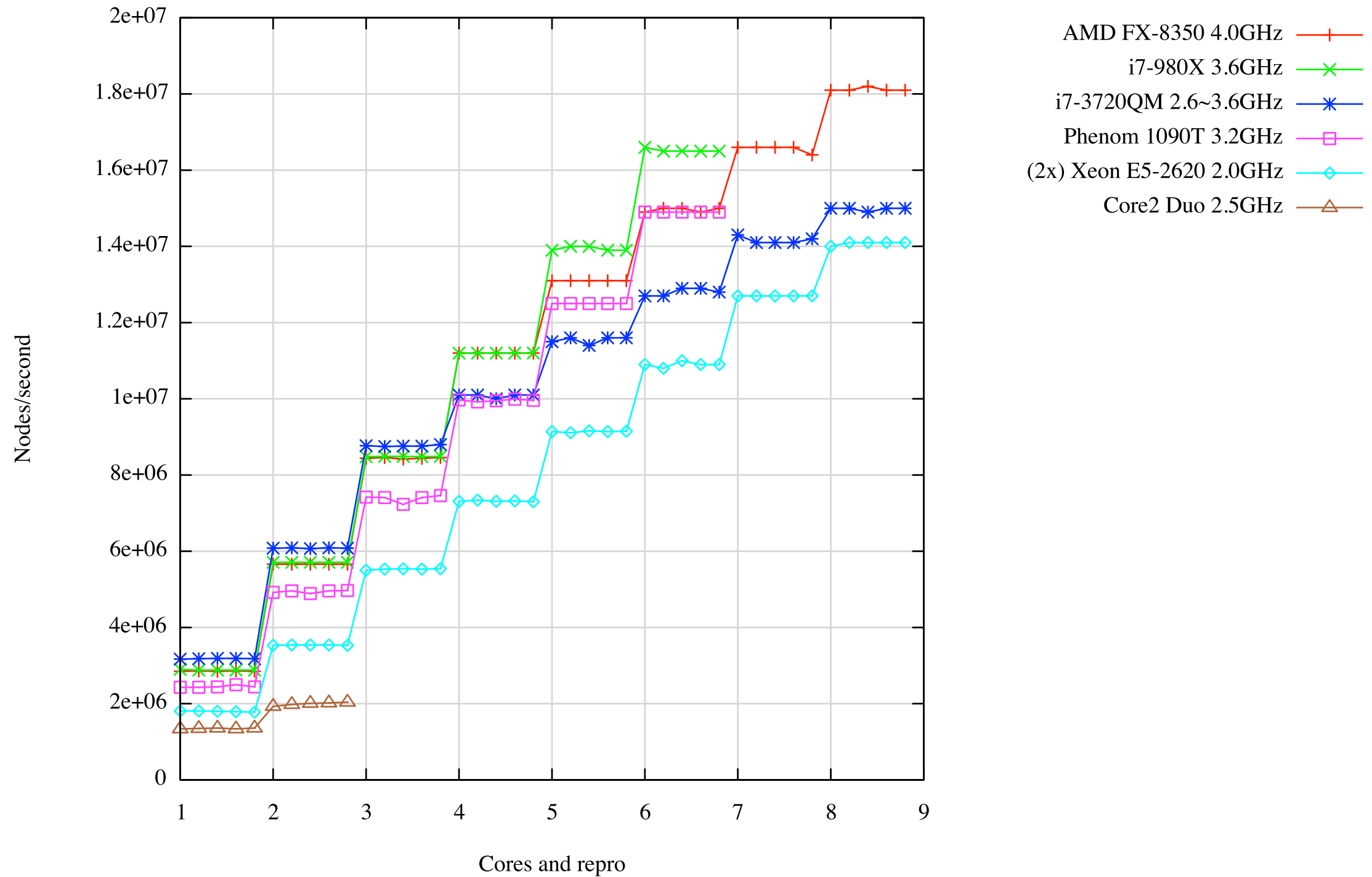
Rookie 3.x - multi-core raw speed benchmark
