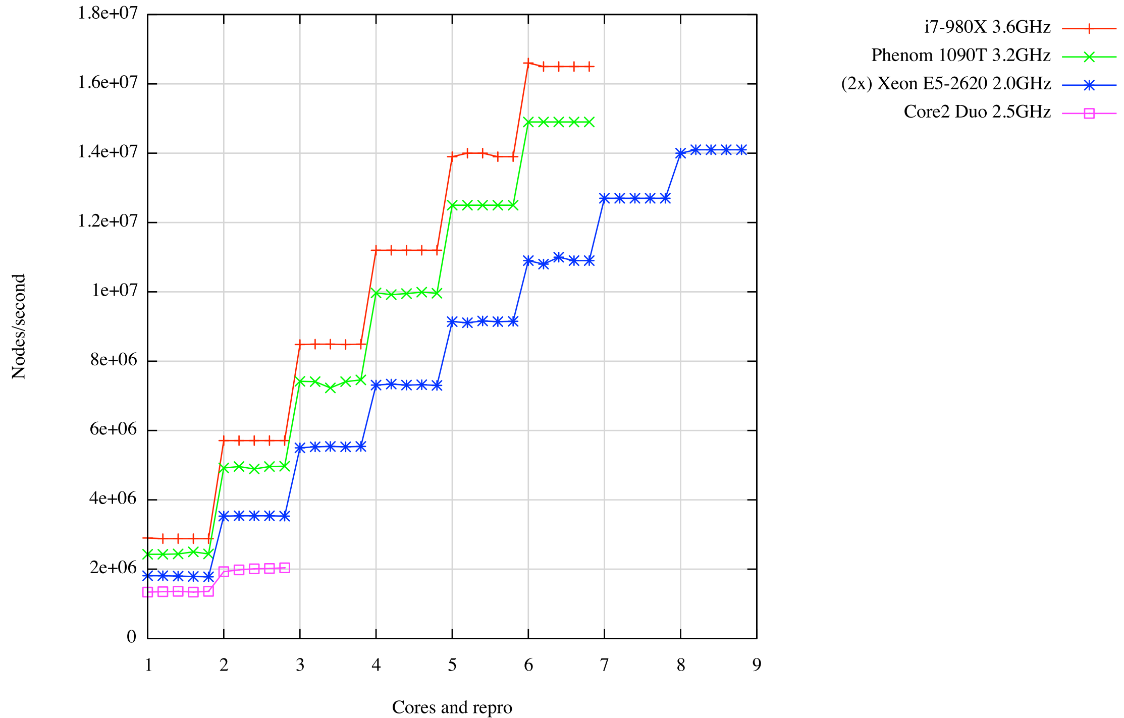
Rookie 3.5b3 - multi-core raw speed benchmark
